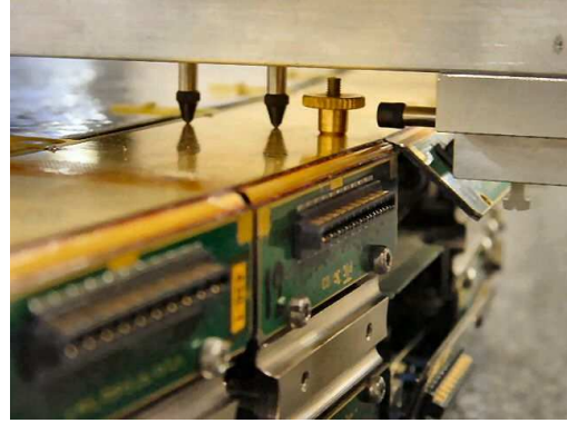
Figure 34. Digital measuring probes held by a rotary arm that are used to measure the dimensions of each eight plane wheel.
