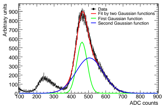
Figure 41. ^{55}\text{Fe} spectrum of a straw with wire offset \sim 600\ \mu\text{m} . Fit of the spectrum by two Gaussian distribution is shown.
